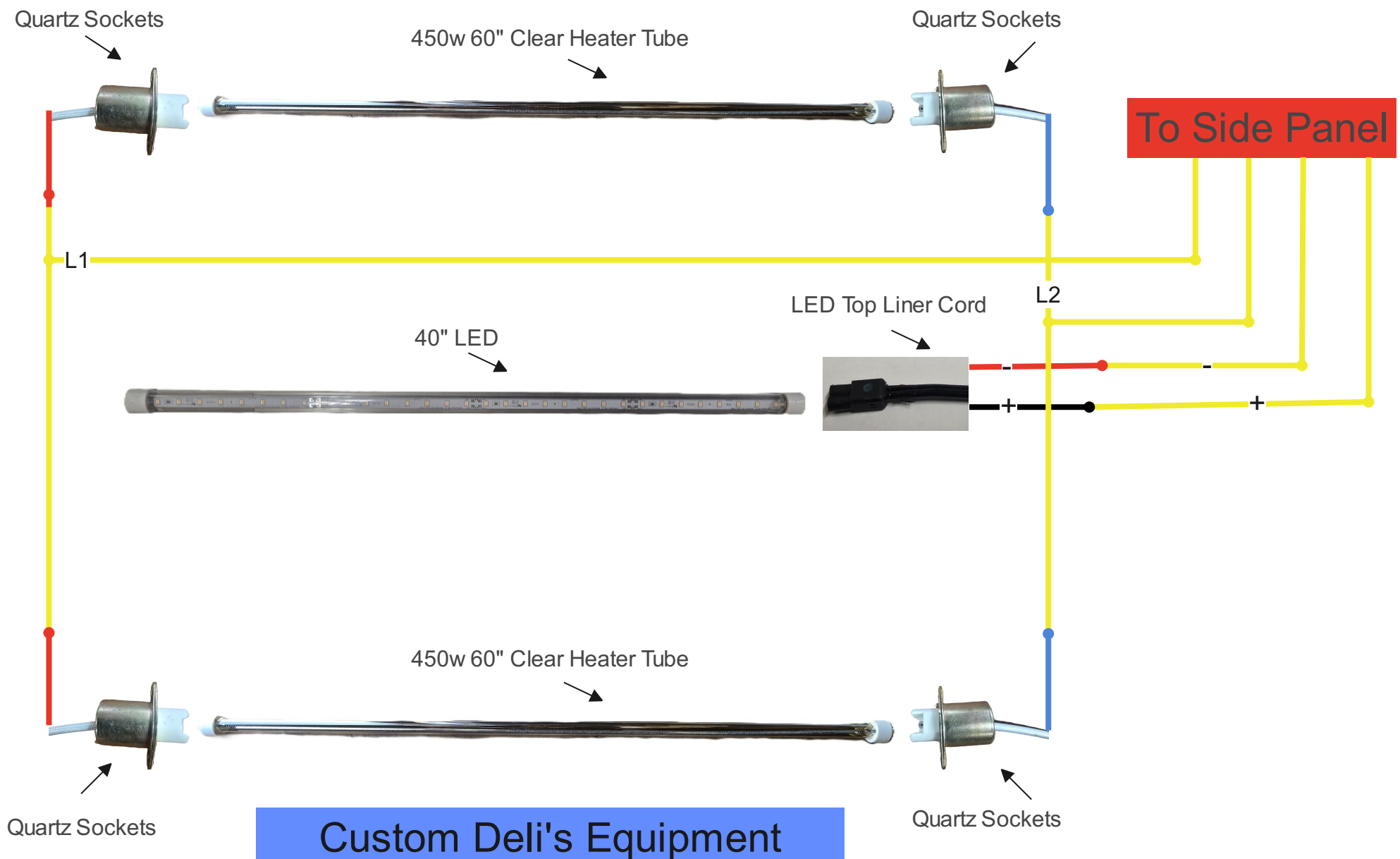
DILW6H 6' 2 Tier FSW Top Liner Diagram
